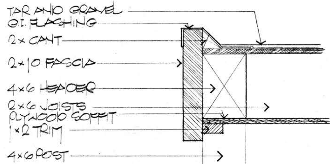
▲ 1 A-3 ROOF AT CARPORT
