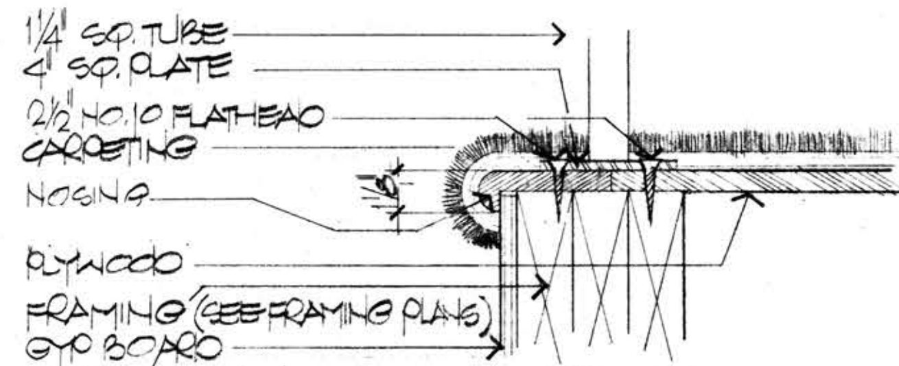
2 A-3 DINING ROOM CURB
