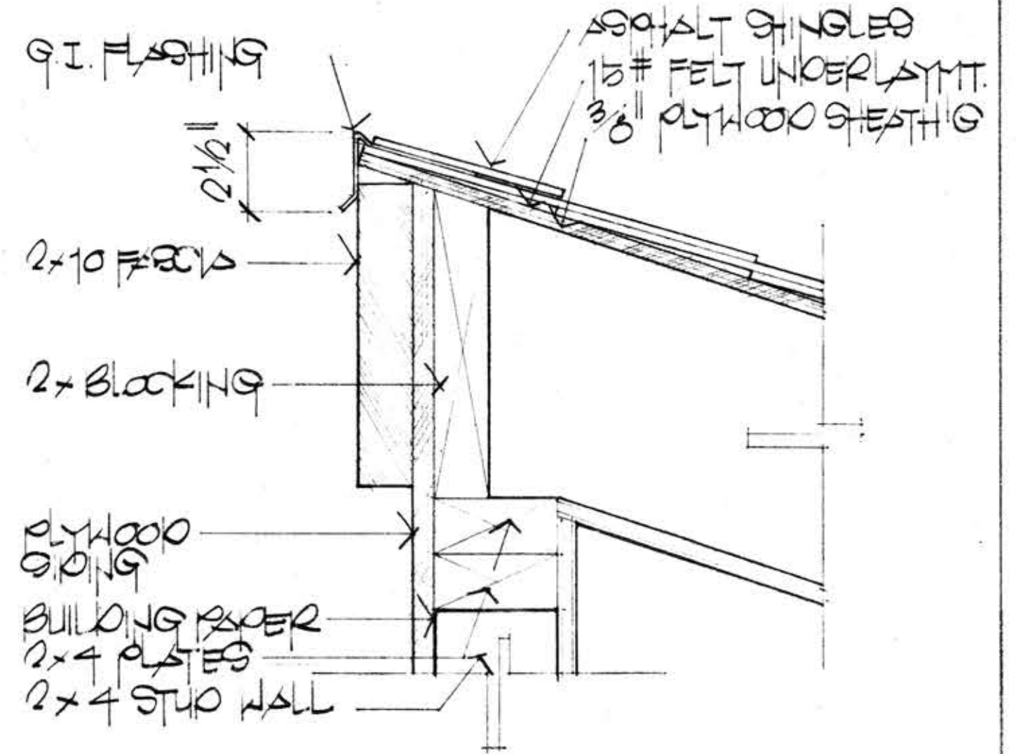
7 A-3 ROOF DETAIL
