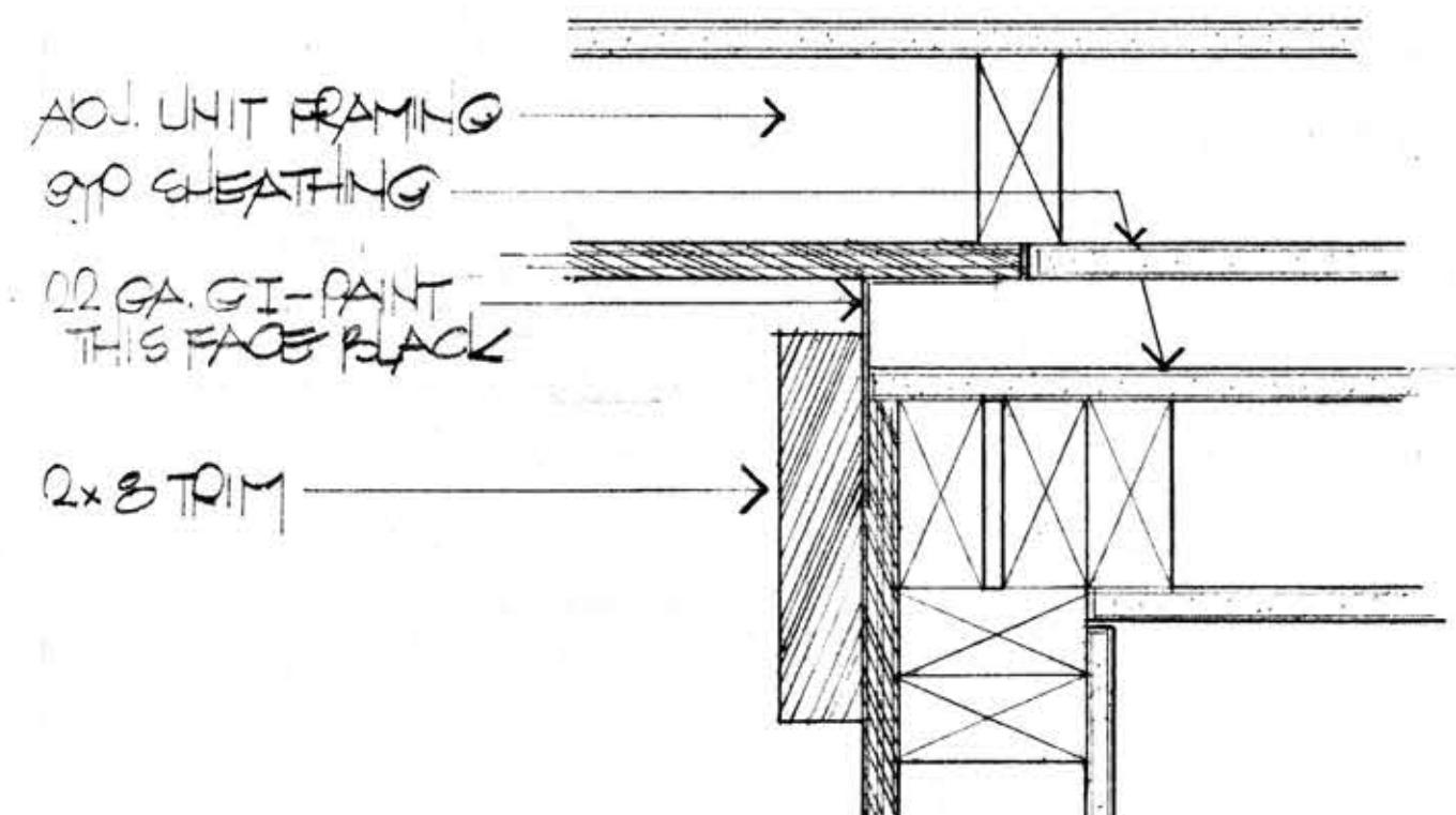
3 A-3 JOINT AT PARTY WALL
