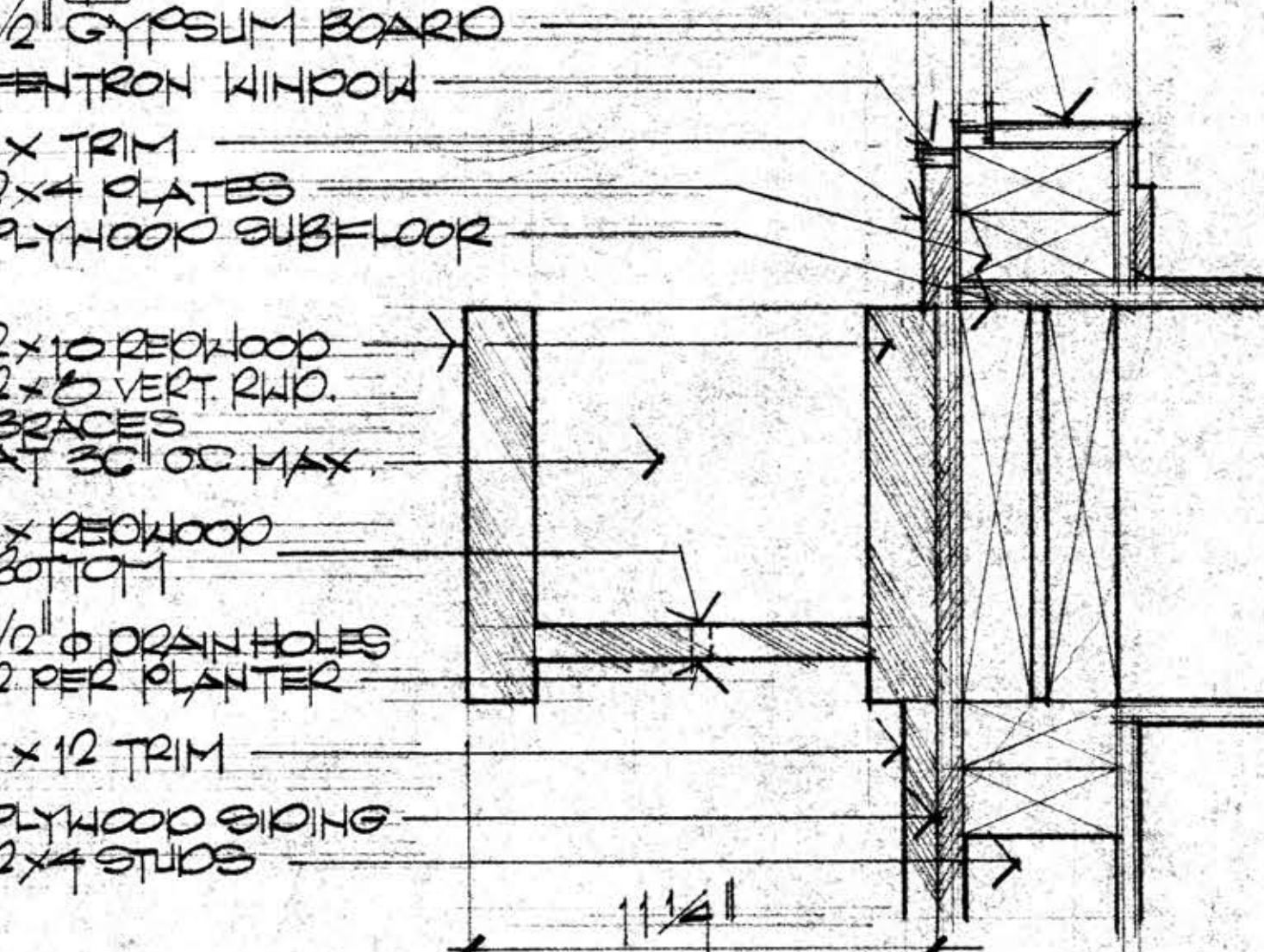
20 PLANTER BOX DETAIL
