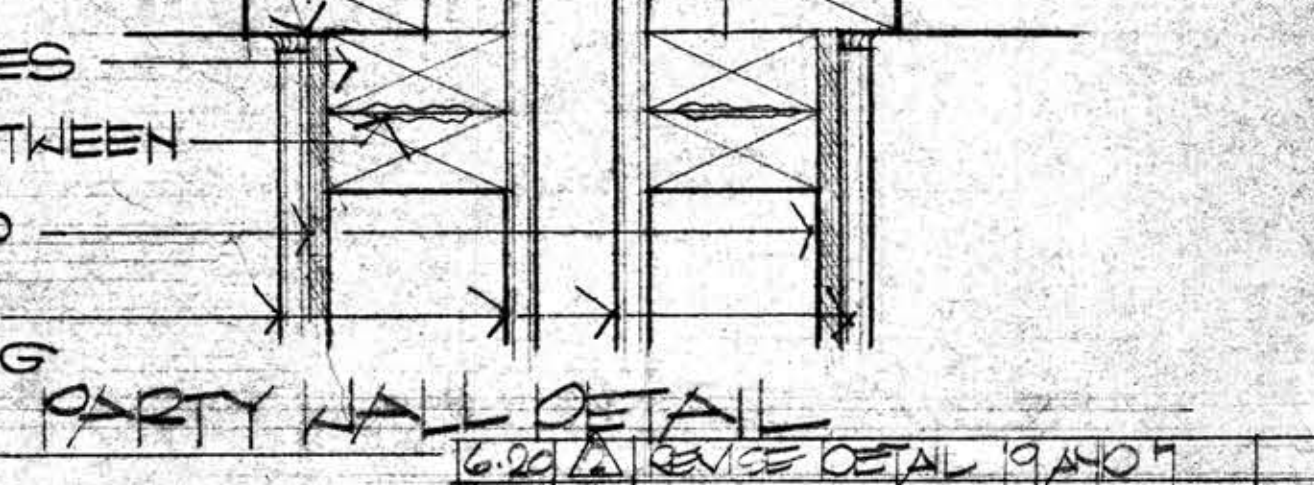
5 PARTY WALL DETAIL
