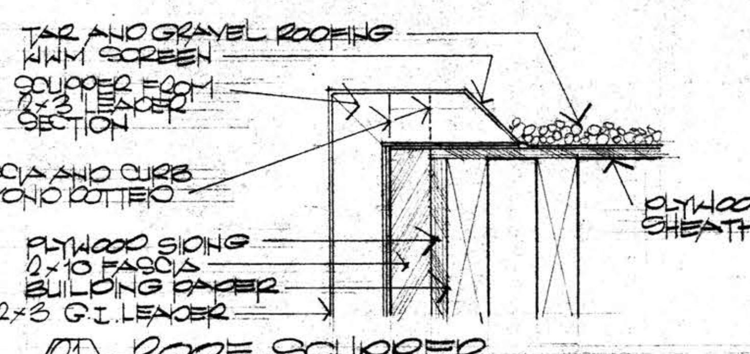
21 ROOF SCUPPER
