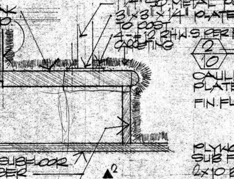
7 STAIR DETAIL
