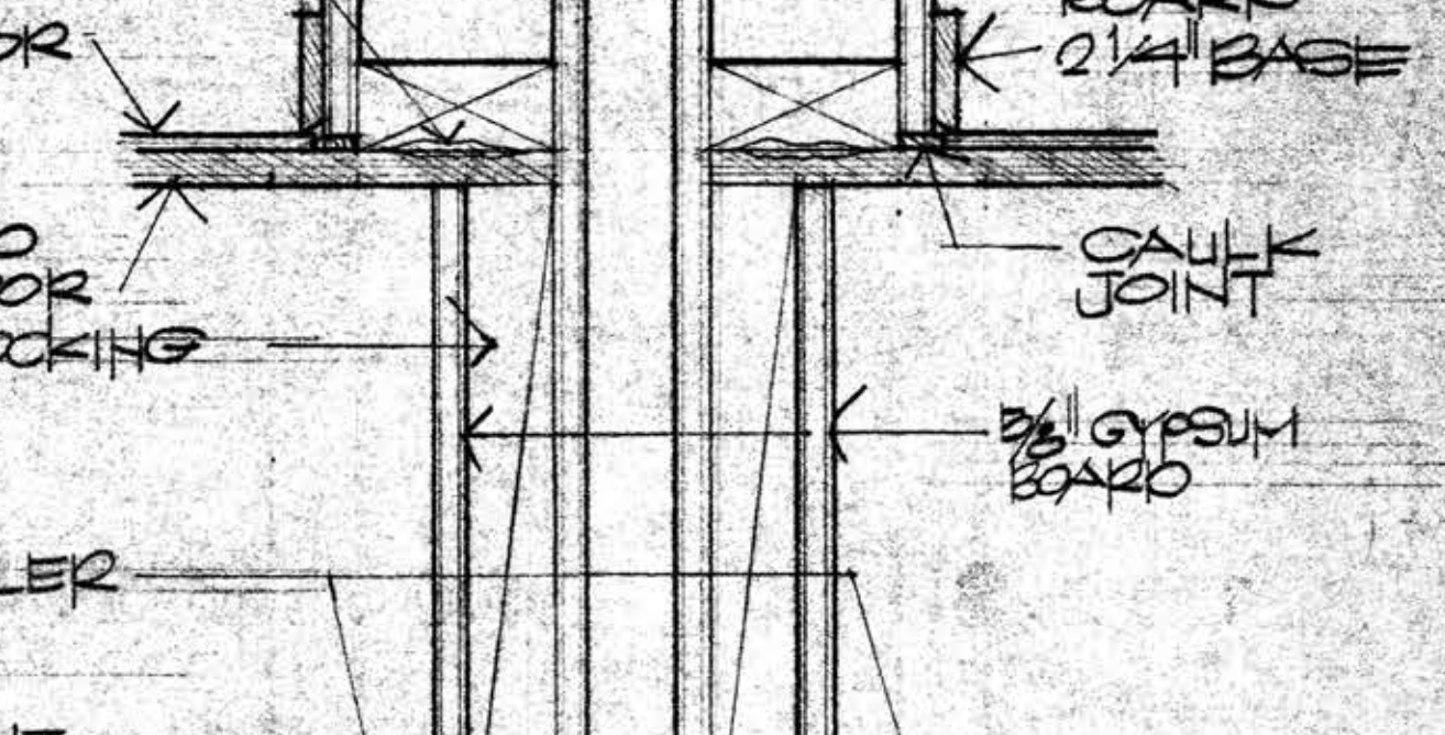
4 PARTY WALL DETAIL
