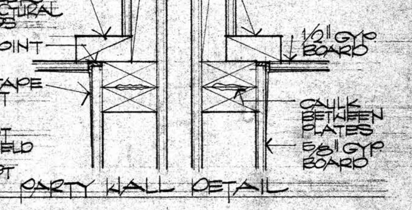
3 PARTY WALL DETAIL
