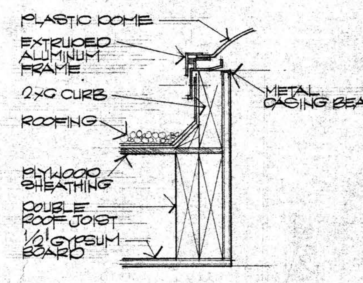
16 SKYLIGHT DETAIL
