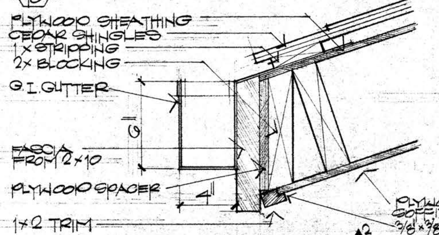
19 GUTTER DETAIL
