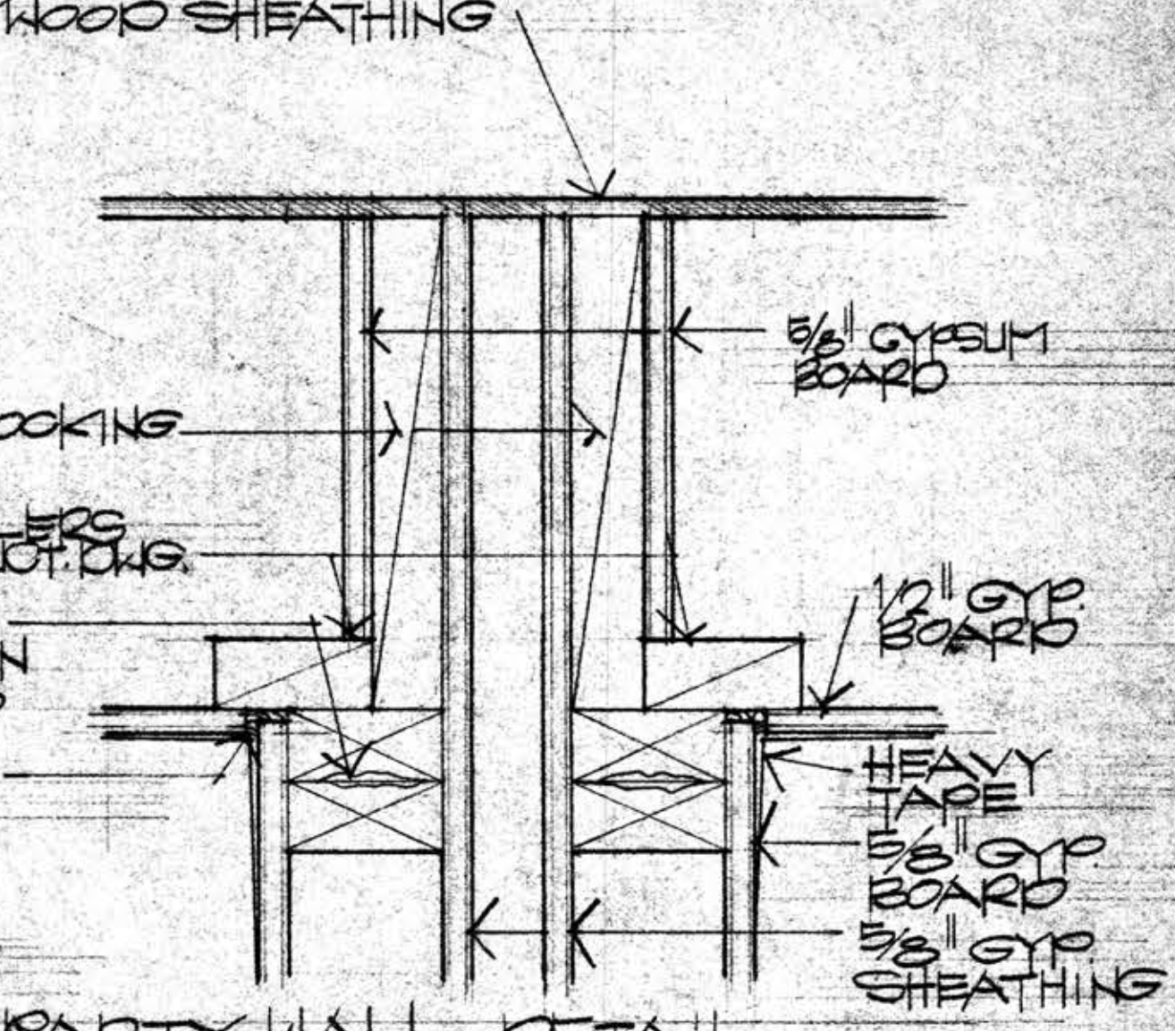
1 PARTY WALL DETAIL
