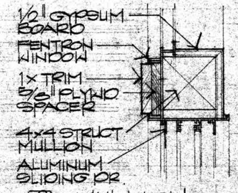
12 MULLION
