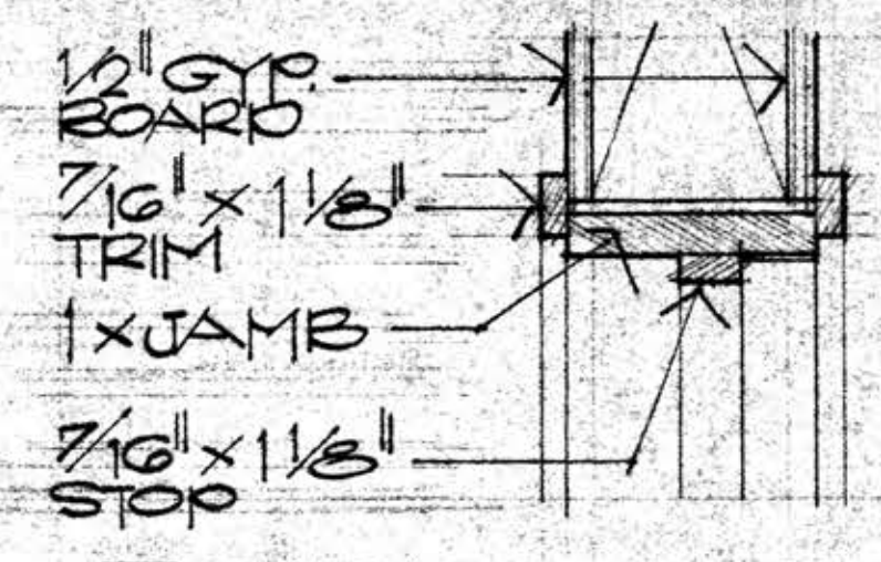
9 HEAD-INTERIOR 10 JAMB SIMILAR
