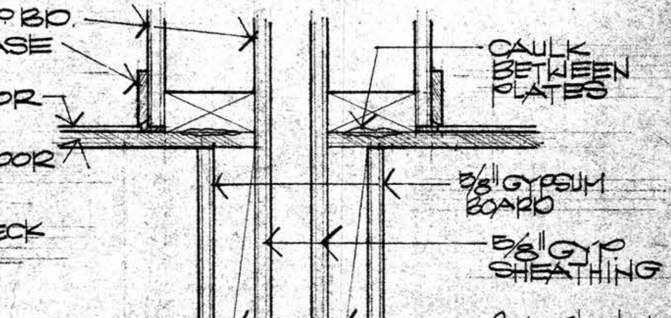
2 PARTY WALL DETAIL
