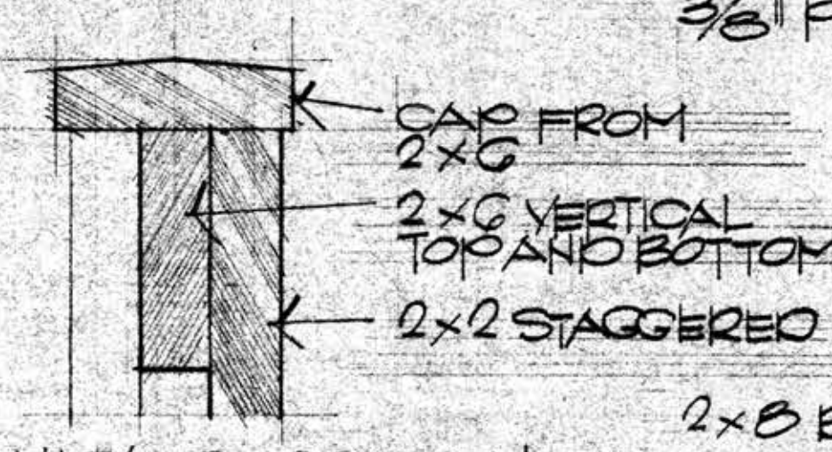
4 HEAD-SCREEN
