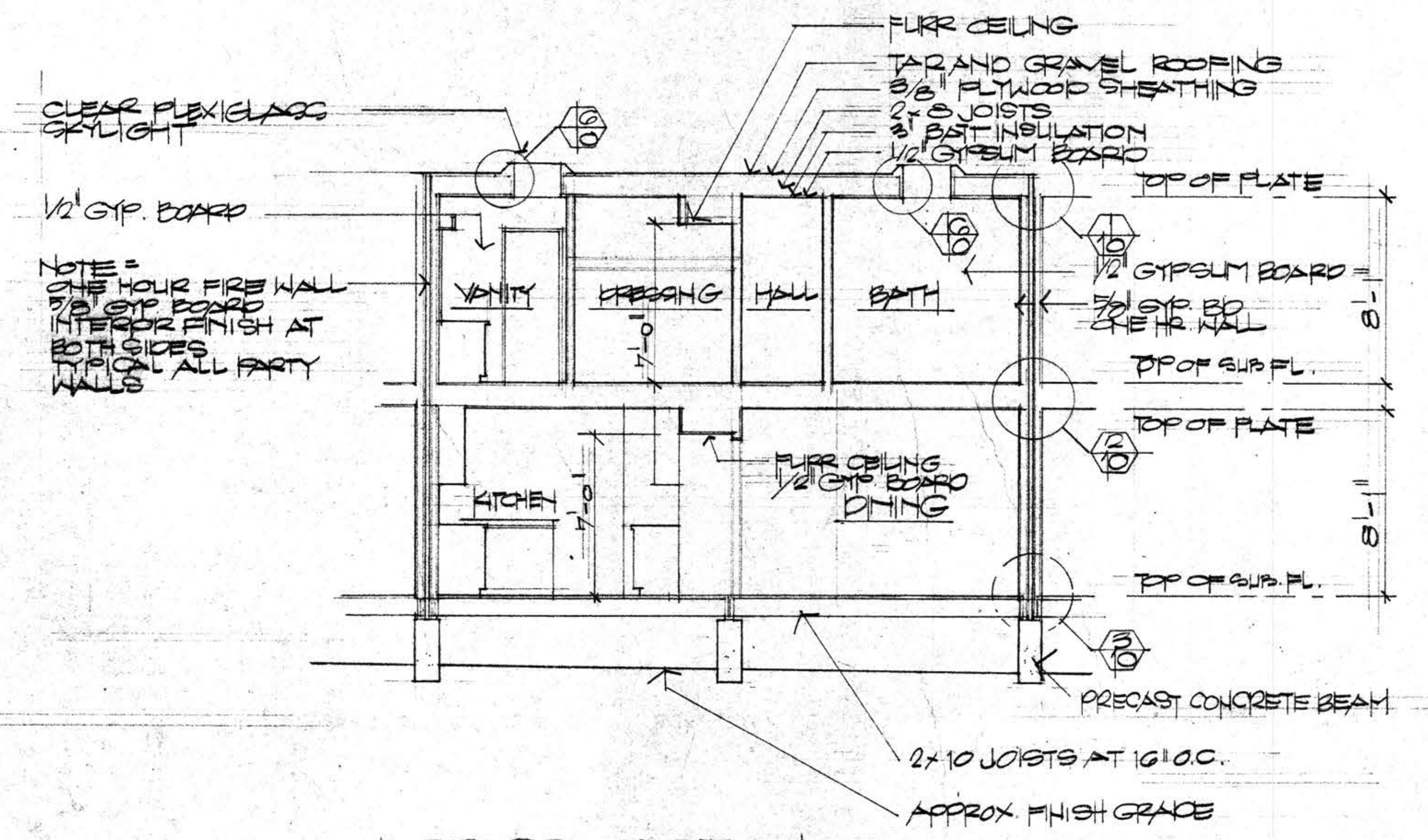
CROSS SECTION
