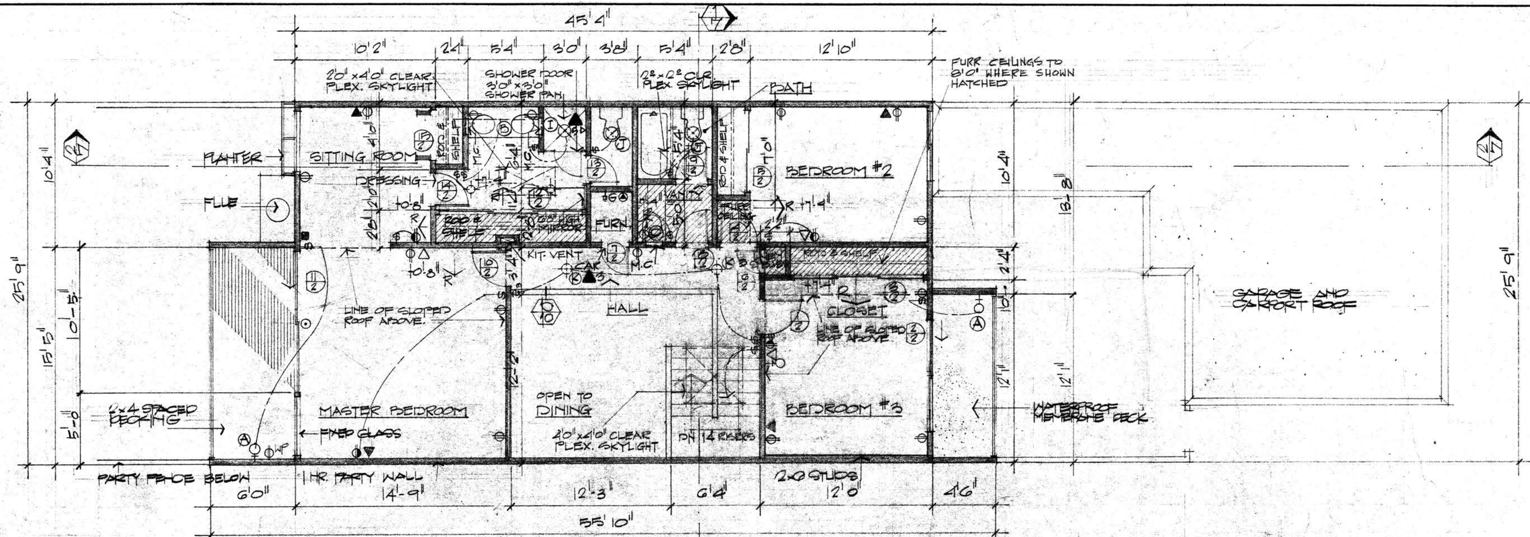
SECOND FLOOR PLAN 1/4" = 1'-0"
