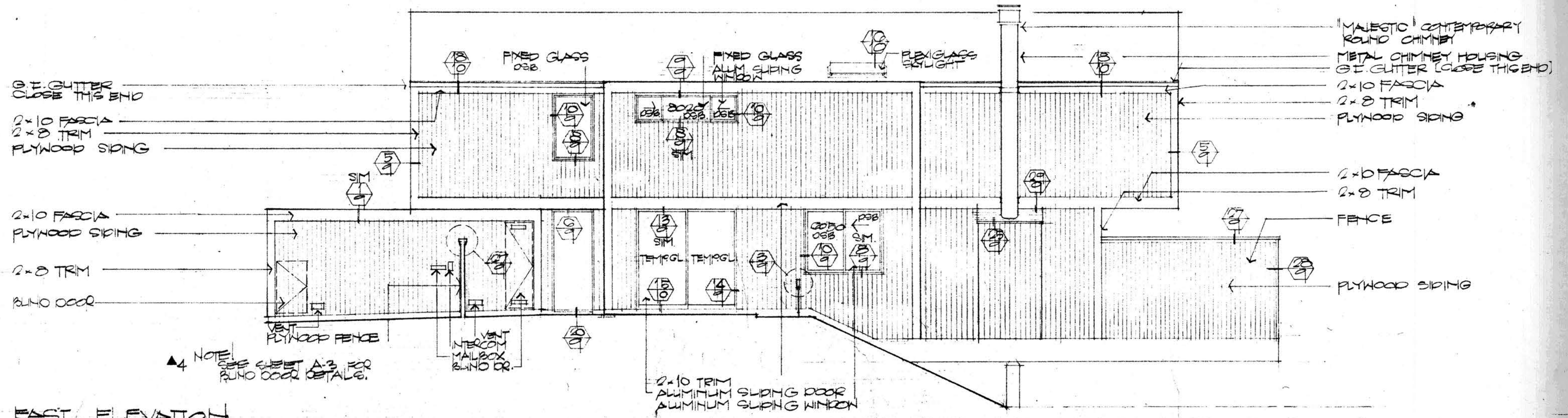
EAST ELEVATION
