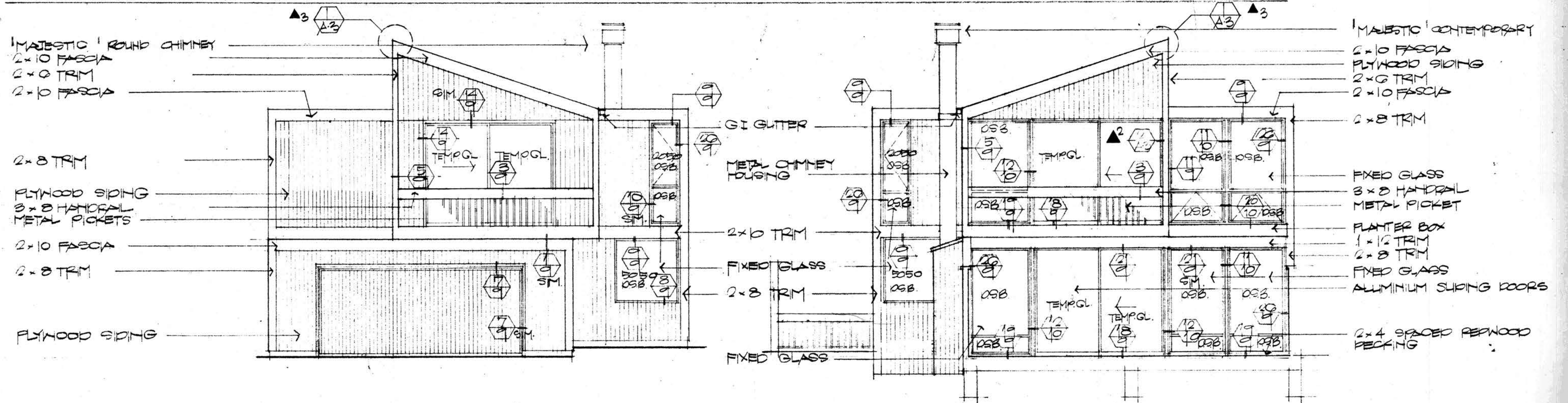
EAST ELEVATION
