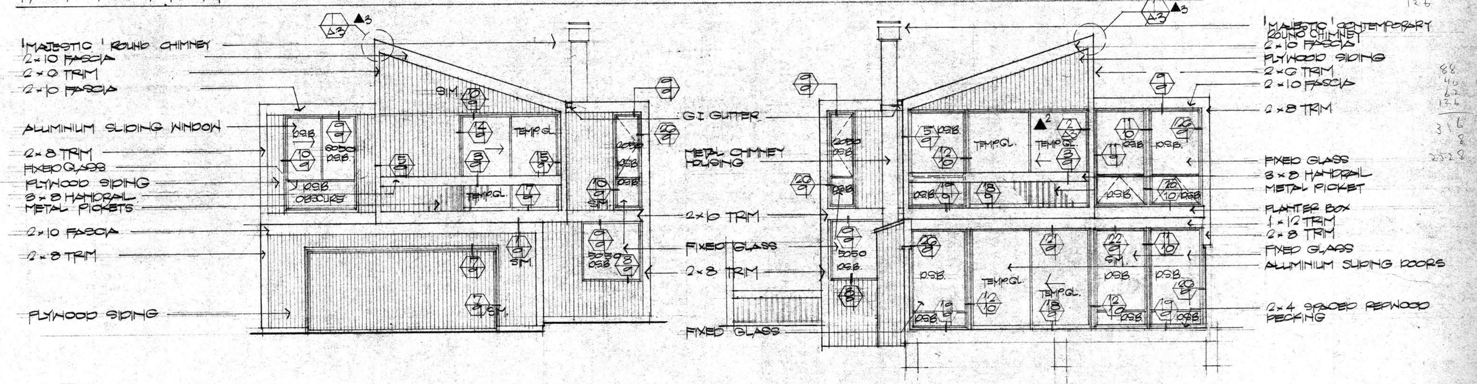
EAST ELEVATION
