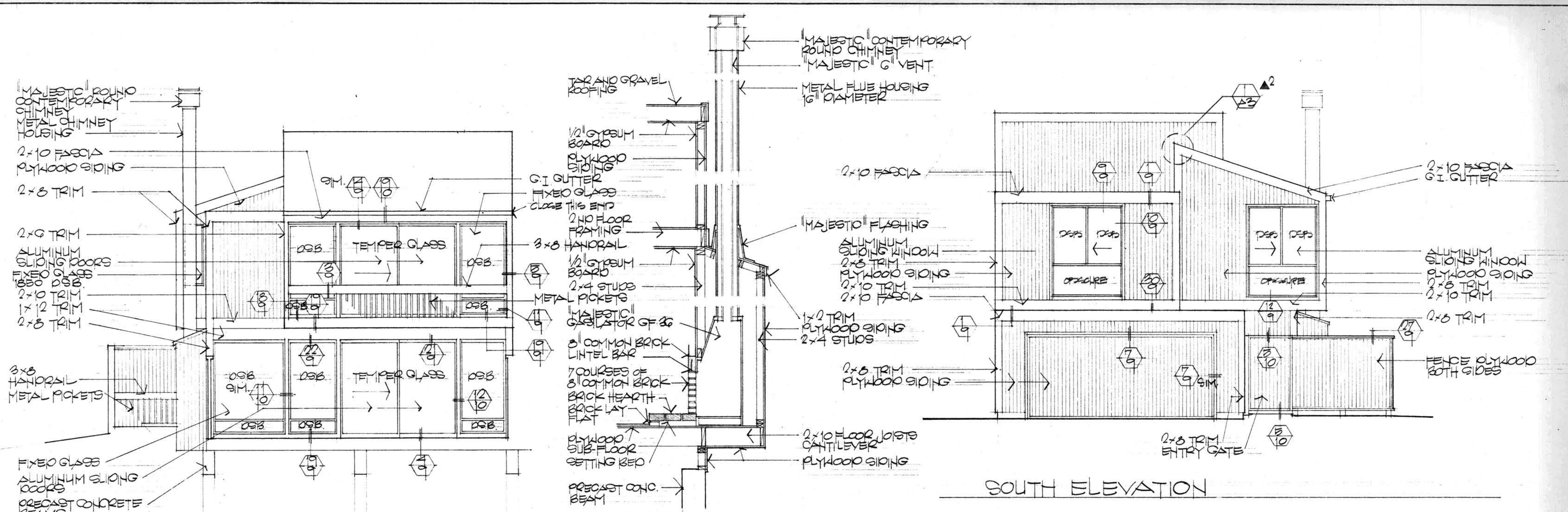
FIREPLACE SECTION
