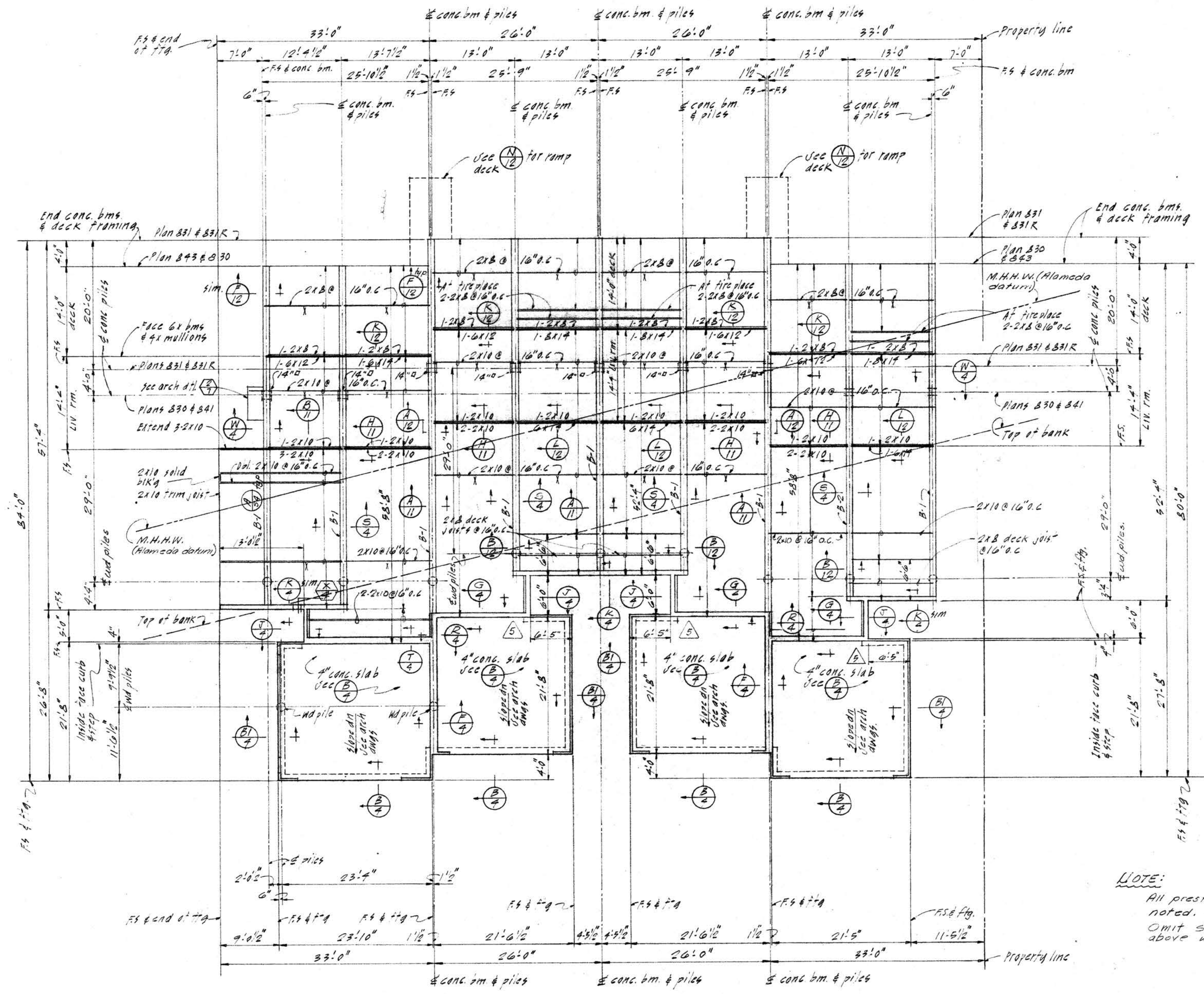
PLAN B43 R LOT 1 BLOCK 3 PLAN B31 LOT 2 BLOCK 3 PLAN B31-R LOT 3 BLOCK 3 PLAN B30 LOT 4 BLOCK 3
